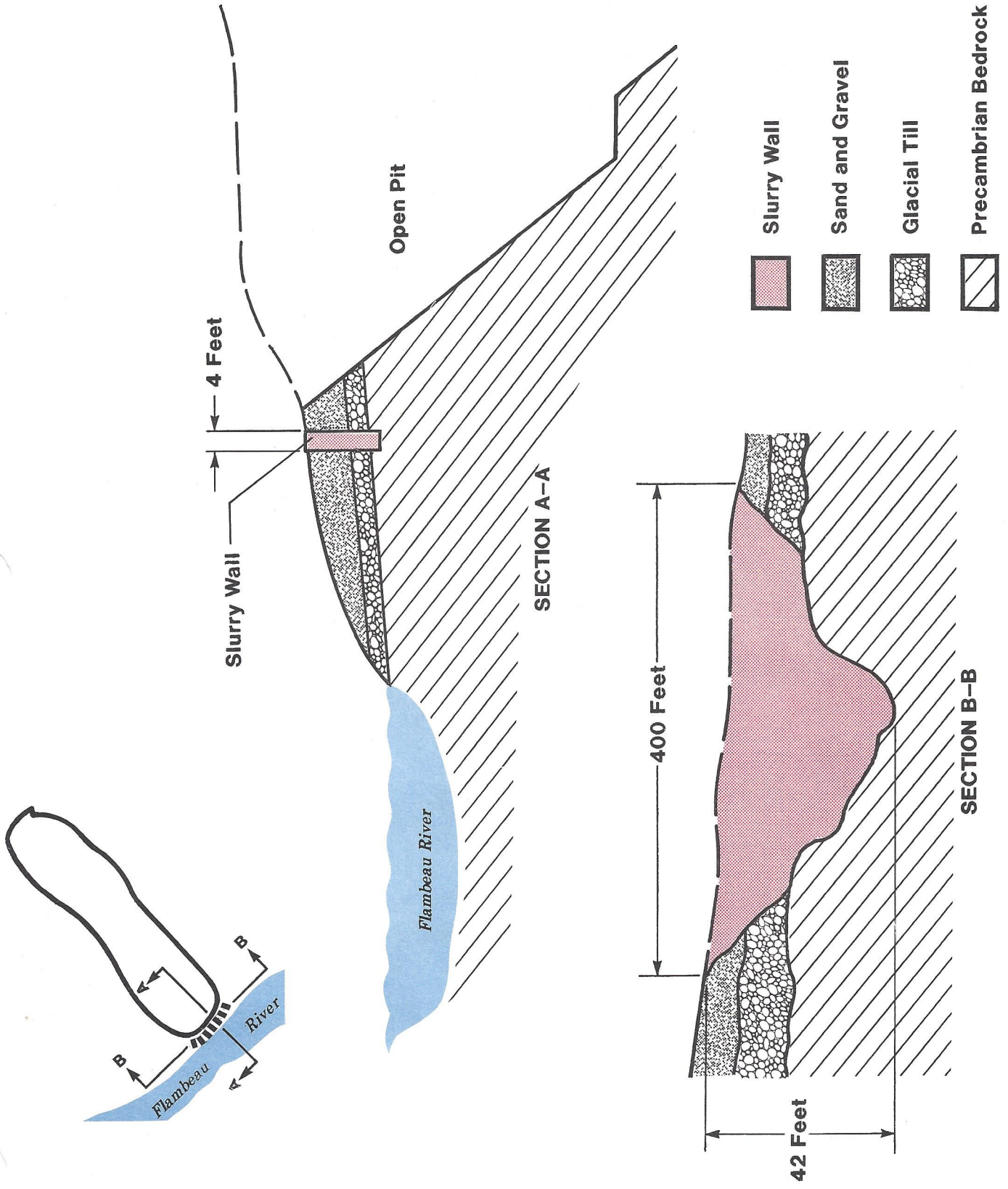
Figure 1-5 Slurry Wall Cross Section
